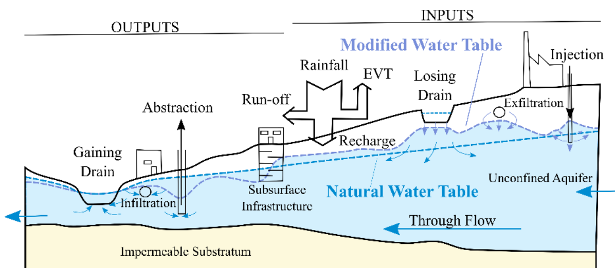
Figure 6-1 Diagrammatic exploration of the impacts of higher groundwater levels in an urban coastal environment (Bosserelle, 2020)
