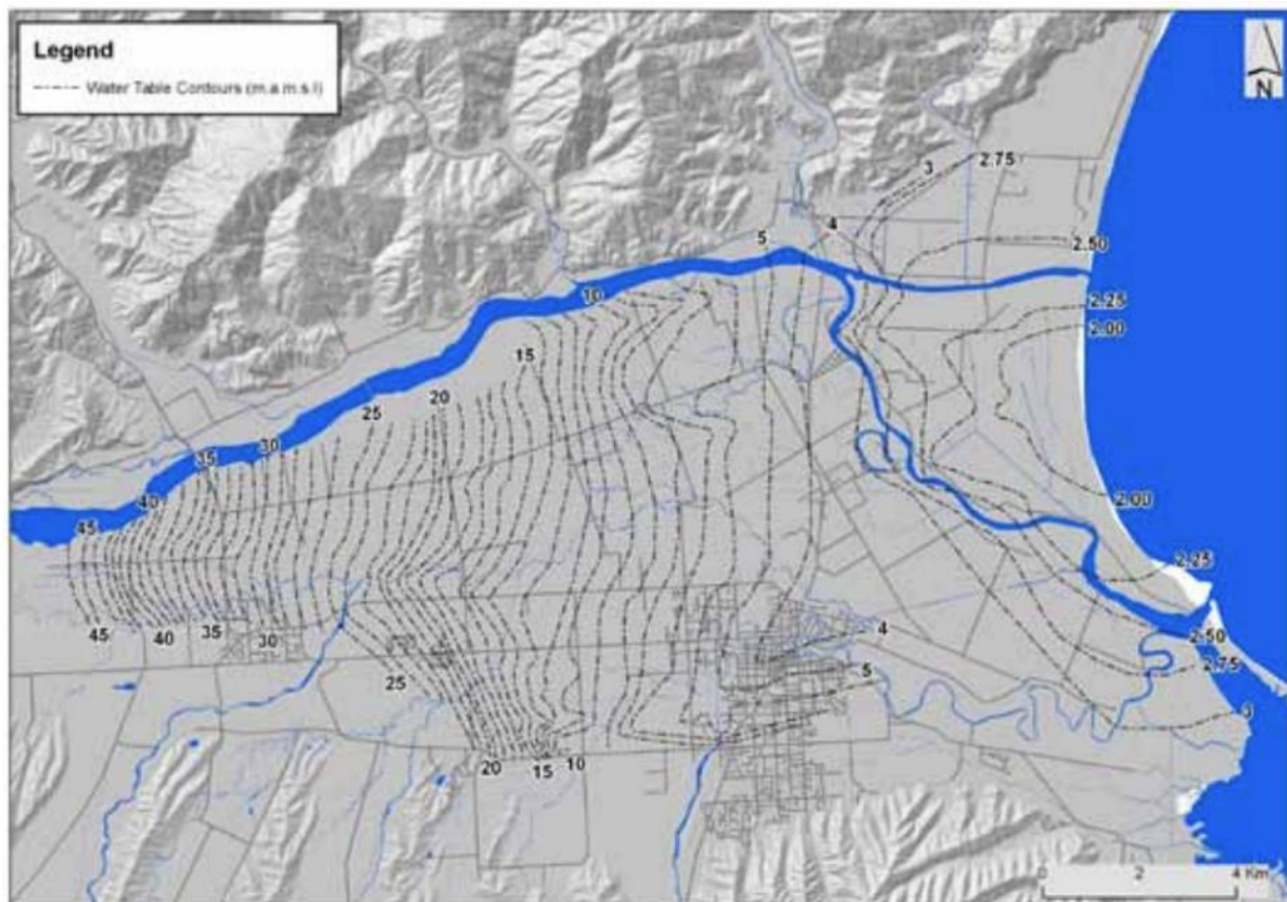
Figure 2-4 Piezometric contours (labels in m msl) based on data collected in March 1978, a relatively dry summer (Davidson & Wilson, 2011)
