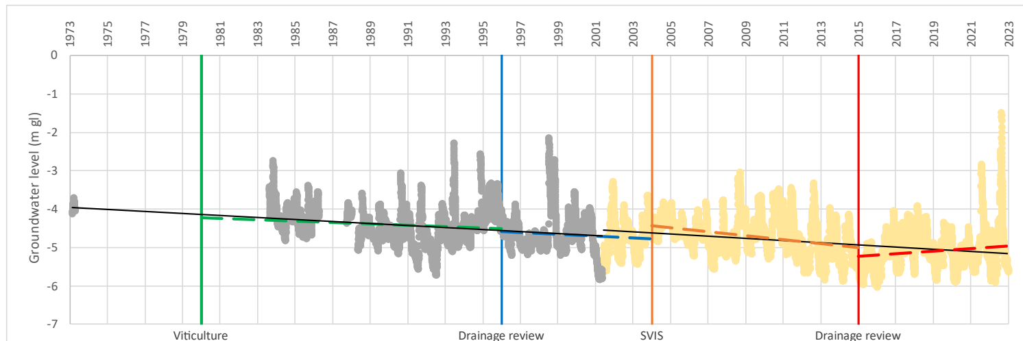
Figure 7-2 Monitoring wells P28w/0398 (grey) and P28w/3821 (yellow) at Condors data, trendline for all data (black), and colour coded significant events that could have impacted groundwater levels (vertical lines as labelled (SVIS: Southern Valleys Irrigation Scheme)), with trendlines in the same colour
