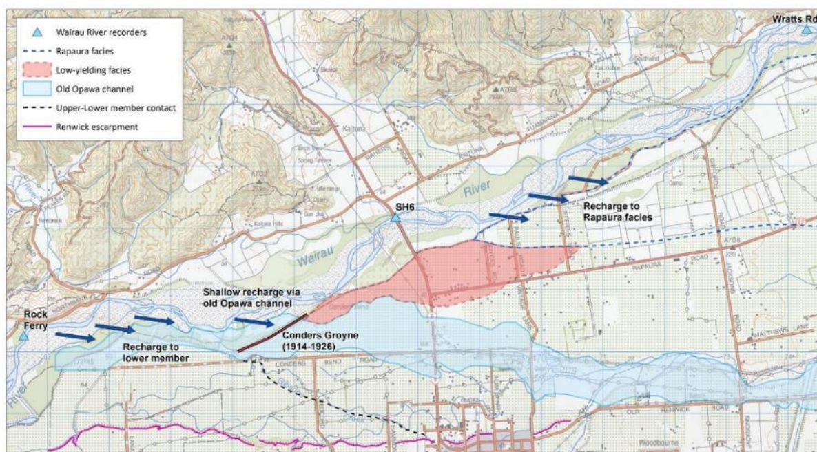
Figure 2-2 Main areas of Wairau Aquifer recharge (Wilson, 2016)
