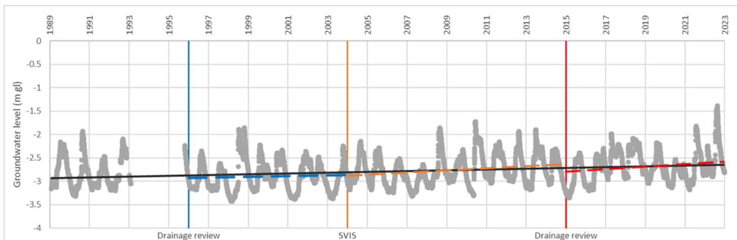
Figure 7-5 Monitoring well P28w/1901-10230 at Rarangi Golf Course data (grey), trendline for all data (black), and colour coded significant events that could have impacted groundwater levels (vertical lines as labelled (SVIS: Southern Valleys Irrigation Scheme)), with trendlines in the same colour
