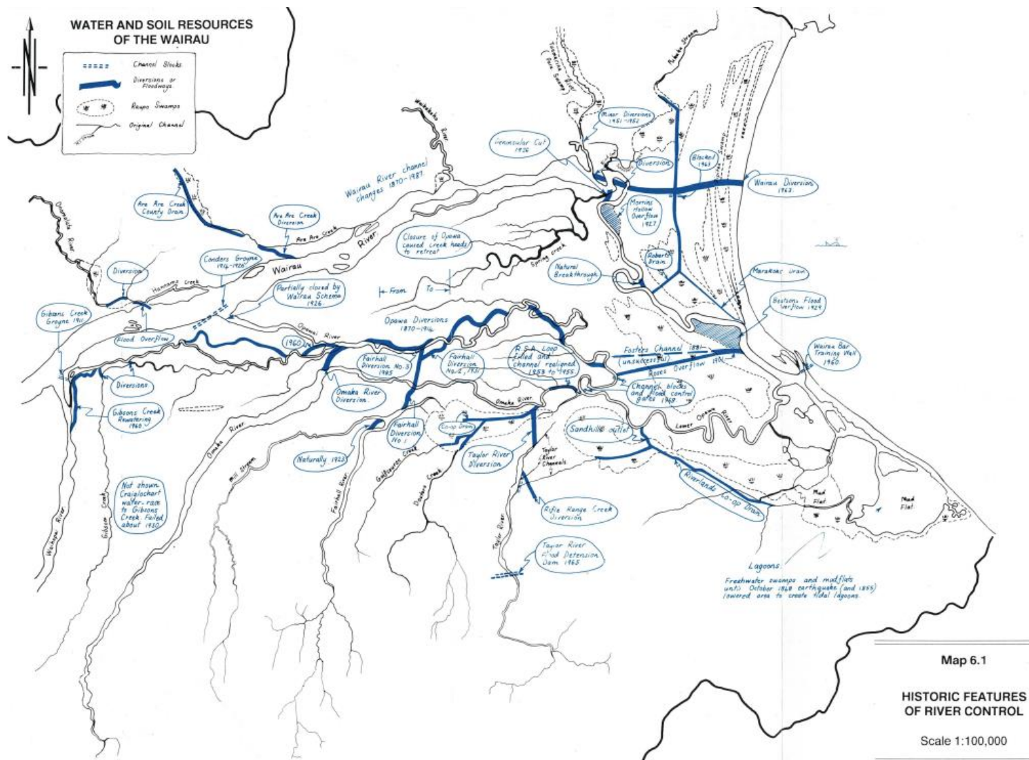
Figure 3-4 Early river management interventions as in Rae (1987). Note: Opawa is Ōpaoa
