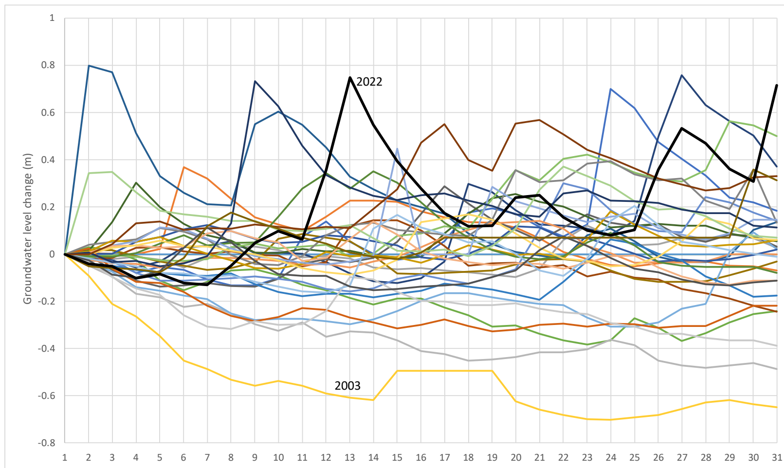
Figure 10-4 Groundwater level change across July by year at Coastal Bar
